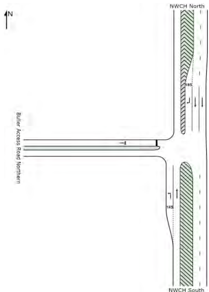
Figure 17: Buller Northern Access Road / NWCH turning lanes
